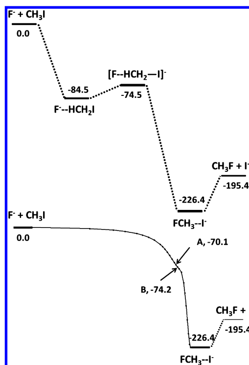
Figure 1. The intrinsic reaction coordinate (IRC) potential energy curve for the \text{F}^- + \text{CH}_3\text{I} \rightarrow \text{CH}_3\text{F} + \text{I}^- reaction 30 (top) and the potential energy curve with the reactive system constrained to a C_{3v} geometry of the reactive system optimized as the \text{F}-\text{C} distance is varied (bottom). Point A has a \text{C}-\text{F} distance equal to that for the prereaction complex on the IRC potential energy curve, and point B has a \text{C}-\text{F} distance equal to that for the transition state on the IRC potential energy curve. For the C_{3v} curve, the only minimum/maximum is the postreaction ion–dipole complex. Calculations are performed at the DFT/B97-1/ECP/d level of theory, 30 and energies are in kJ/mol.
