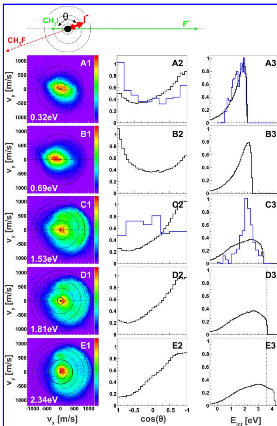
Figure 2. (A1)–(E1) Measured velocity images of the I^- product from reactive scattering of F^- and CH_3I at different collision energies (see the schematic Newton diagram in the center-of-mass frame at the top). The dashed ring with the largest radius in each image represents the kinematical cutoff for the S_N2 reaction with no product excitation. The smaller rings represent spheres of increasing product internal excitation, spaced at 1 eV intervals. The solid circle and the vertical line in panels D1, E1 and D3, E3 indicate the threshold energy for breakup into CH_2 + HF . (A2)–(E2) and (A3)–(E3) Histograms of the scattering angle and the internal excitation (black) for the same relative collision energies as in (A1)–(E1). The E_{int} histograms show a sharp upper bound, caused by products with vanishing velocity, and a more diffuse lower bound, due to the finite energy resolution. Simulation results for 0.32 and 1.53 eV are shown in blue.
