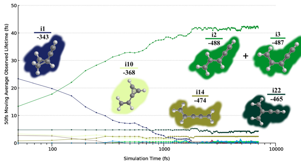
Fig. 6 The population of the six most important intermediates after the collision. The x-axis is in log scale. The number under the intermediate name is the relative energy. The population of i2 and i3 are plotted together instead of separately due to their fast interconversion.
