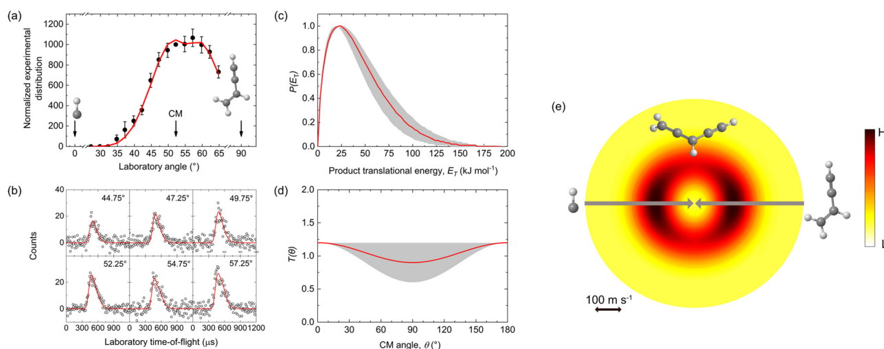
Fig. 1 Laboratory angular distributions of the products recorded at m/z = 63 (C 5 H 3 + ) for the reaction of the methylidyne radical with vinylacetylene (a). The solid circles represent the experimental data. CM designates the center-of-mass angle, the error bars represent the 1 \sigma standard deviation and red solid lines represent the overall fit. Selected TOF spectra are presented in panel (b); open circles depict the experimental data and the solid lines the fit. Center-of-Mass (CM) translational energy distribution P(E_T) (c) and angular distribution T(\theta) (d) along with the associated flux contour map (e) leading to the formation of ethynylallene ( p1 ). Shaded areas indicate the error limits of the best fits accounting for the uncertainties of the laboratory angular distribution and TOF spectra, with the red solid lines defining the best-fit functions. The flux contour map represents the flux intensity of the reactive scattering products as a function of the CM scattering angle ( \theta ) and product velocity ( u ). The color bar indicates the flux gradient from high ( H ) intensity to low ( L ) intensity. Atoms are color coded as follows: carbon (black), and hydrogen (grey).
