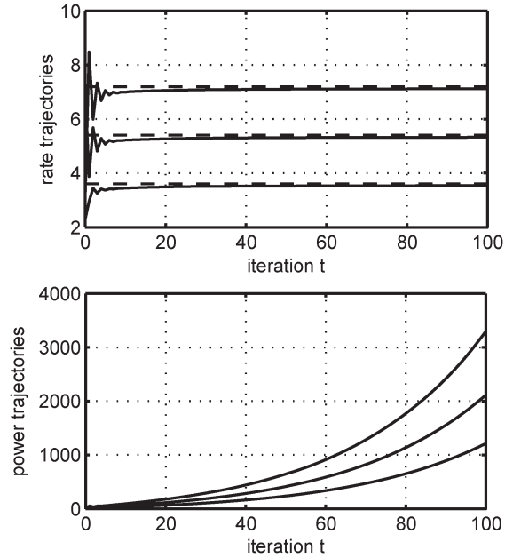
Fig. 3. Rate and power trajectories generated by (24) with \bar{u}^2 .
