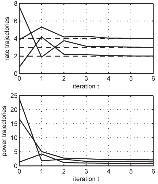
Fig. 2. Rate and power trajectories generated by (24) with \bar{u}^1 .
