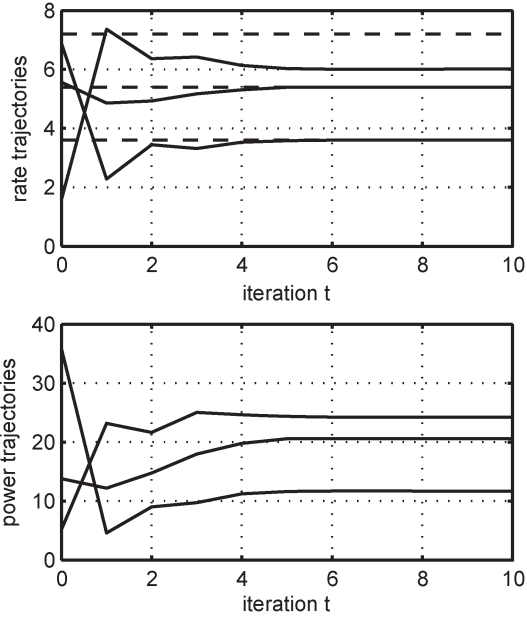
Fig. 4. Rate and power trajectories generated by (23) with \bar{u}^2 .
